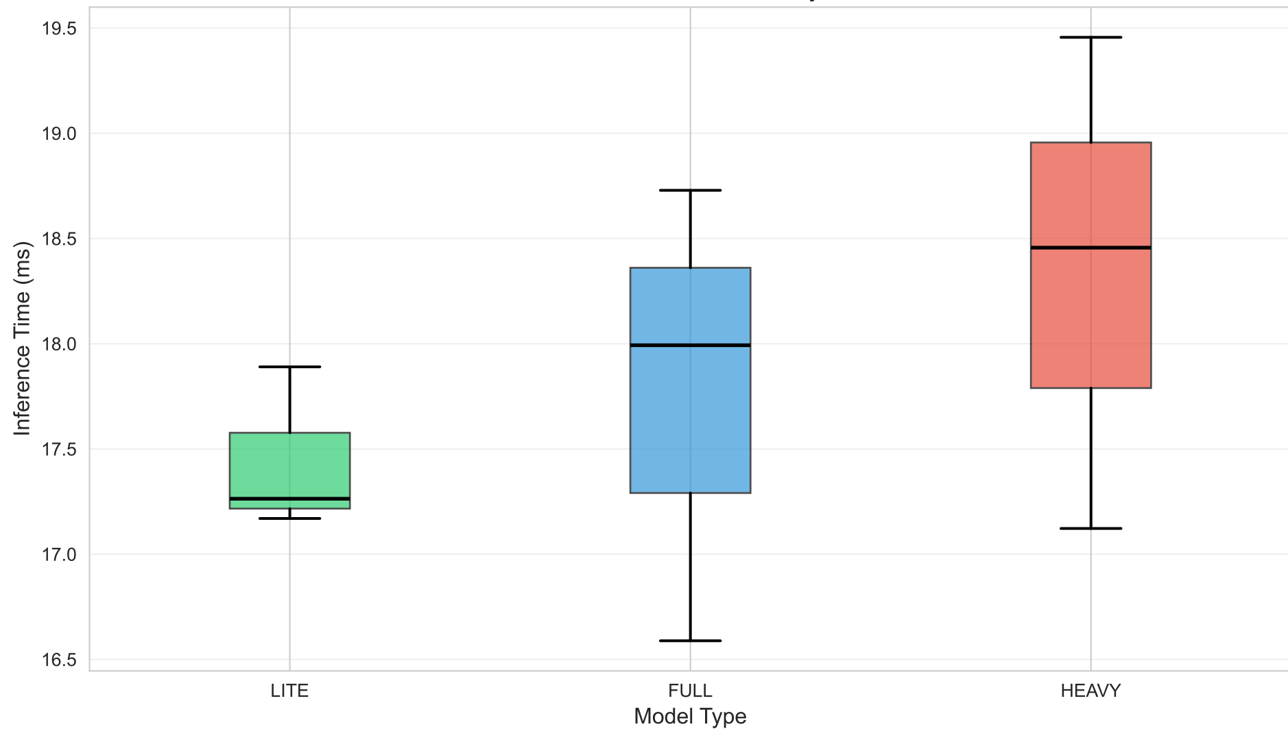
Inference Time Distribution by Model
